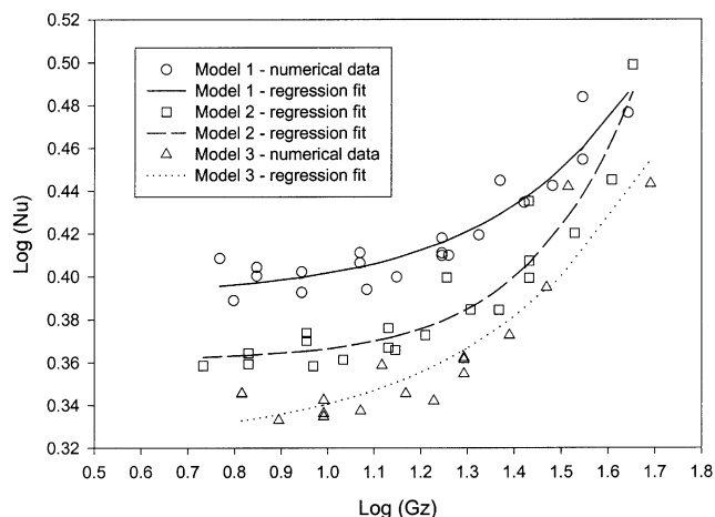
Fig. 5. Nu vs Gz values for straight edge of channel.
